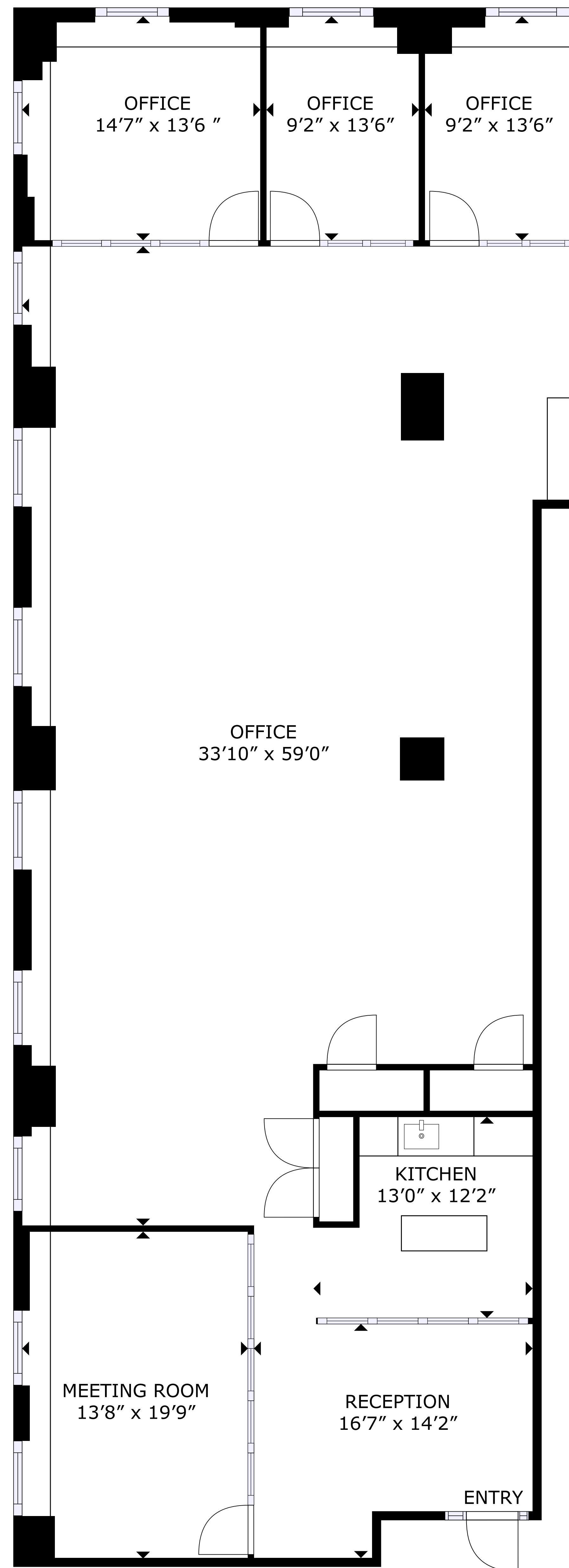
FLOOR PLAN
